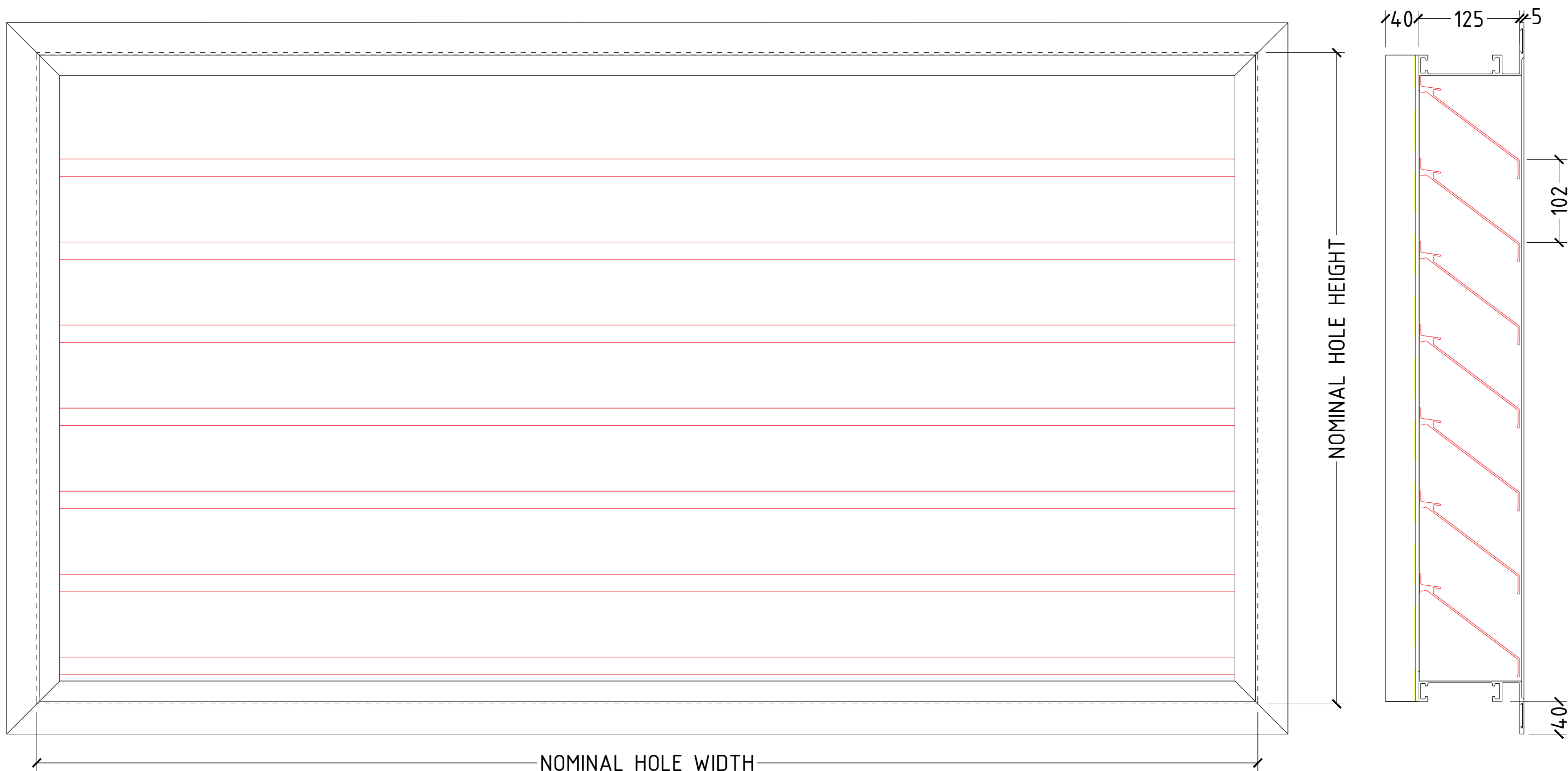
SIDE ELEVATION
