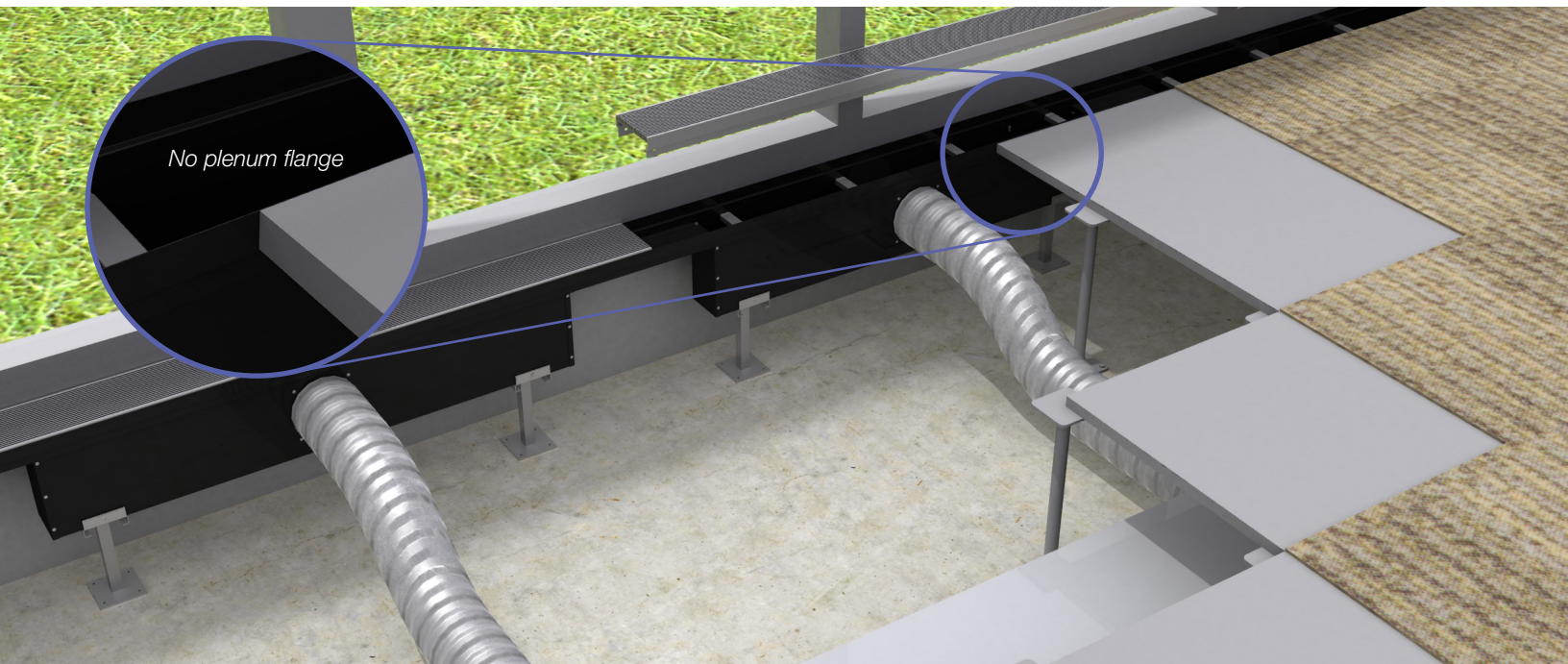
LFP with pedestal supported assembly
